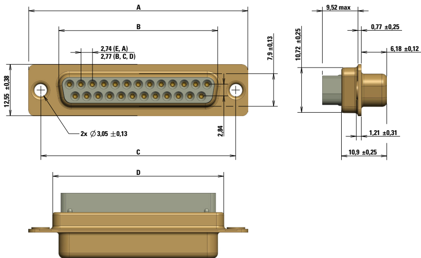
Socket connector dimensions - Sizes E-A-B-C
