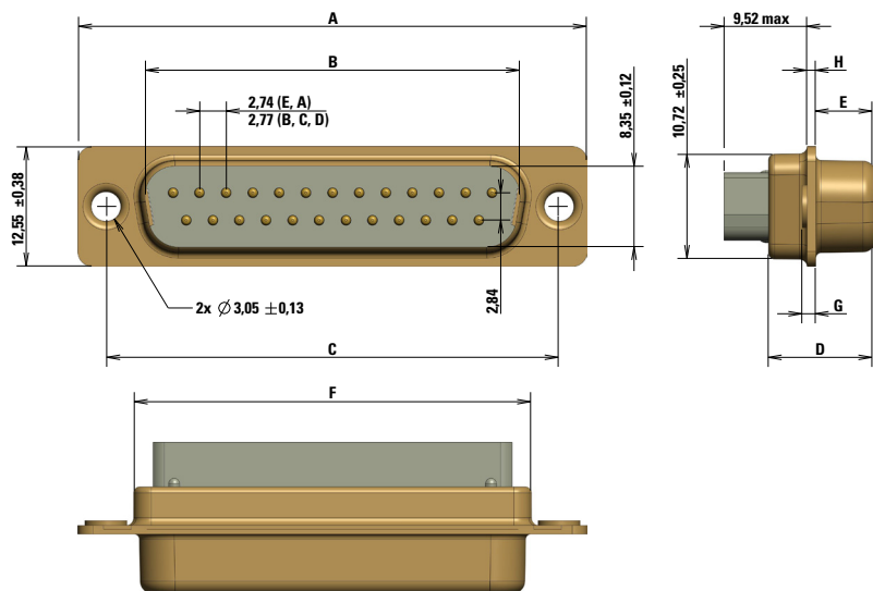
Pin connector dimensions - Sizes E-A-B-C
