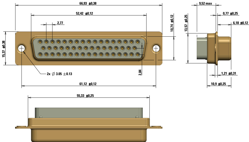
Socket connector dimensions - Size D
