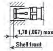
Female contact
