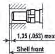
Male contact
