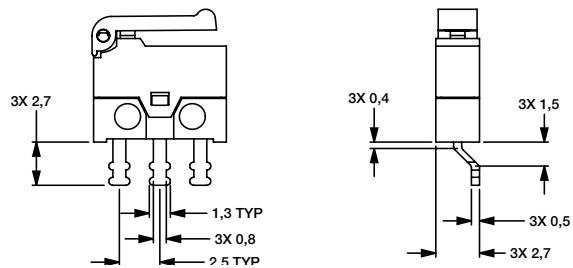
SR SMT, Right Mount
