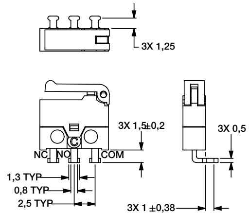
LS PC Thru-hole, Short Left Bend
