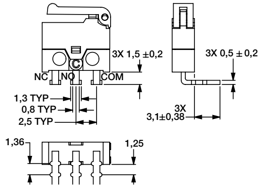
LL PC Thru-hole, Long Left Bend
