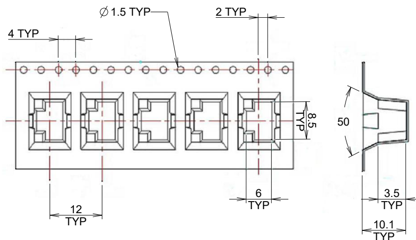
SV SMT, Vertical Mount
