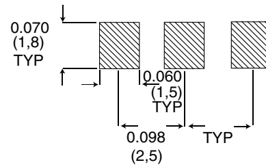
SMT Mounting Pattern
