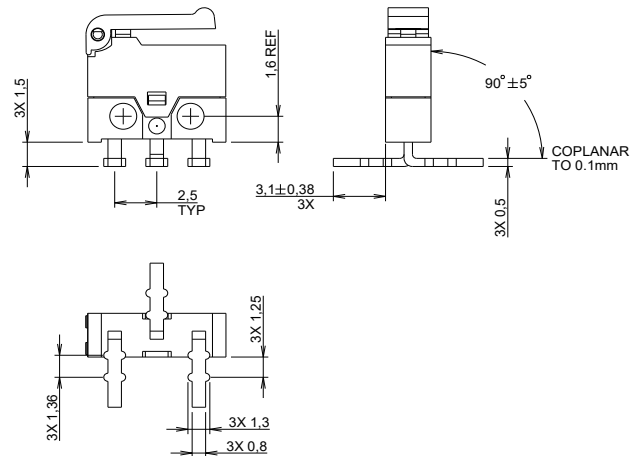
SV SMT, Vertical
